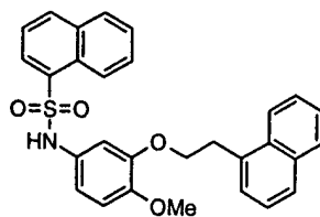
Compound # 50
